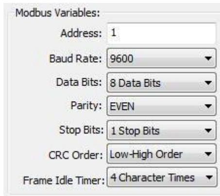
Figure 2.6 Modbus communication parameters
